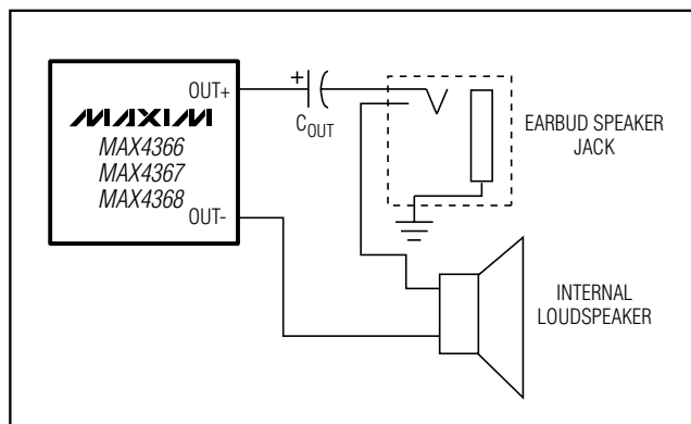
Figure 7. Headset with Internal Speaker Application Circuit
