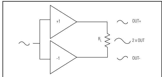
Figure 1. Bridge-Tied Load Configuration
