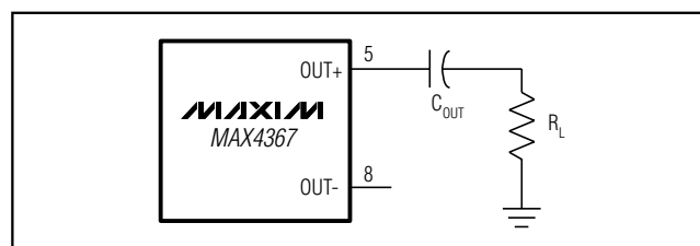
Figure 2. MAX4367 Single-Ended Configuration
