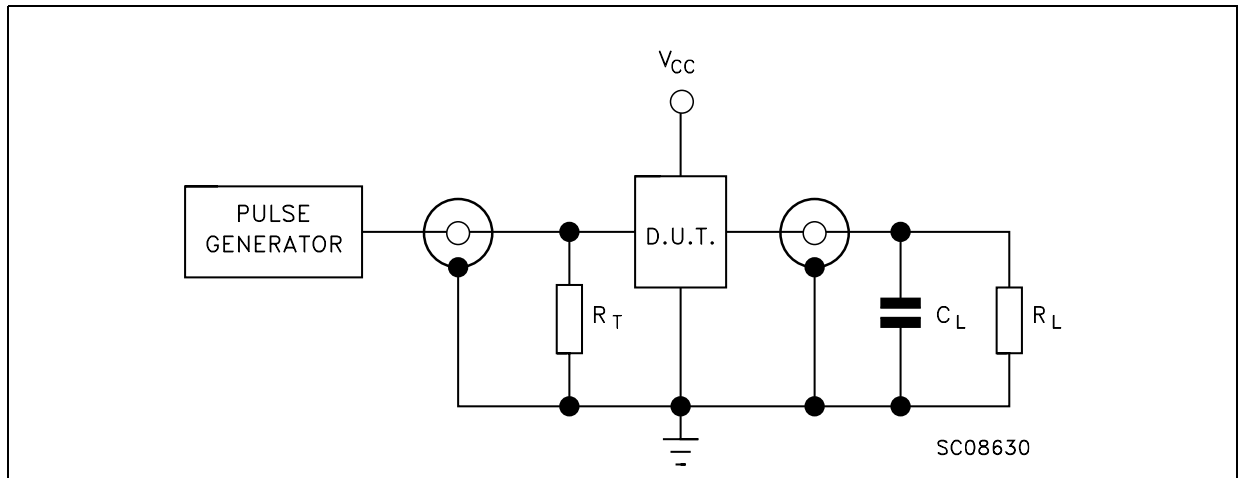
Figure 8. Test circuit
