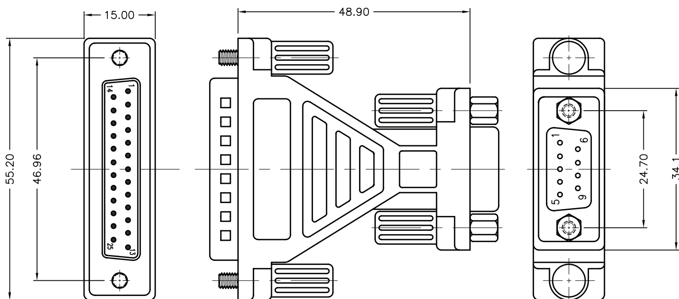
DB-25 Pin Male
