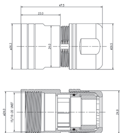
Cord Grips
