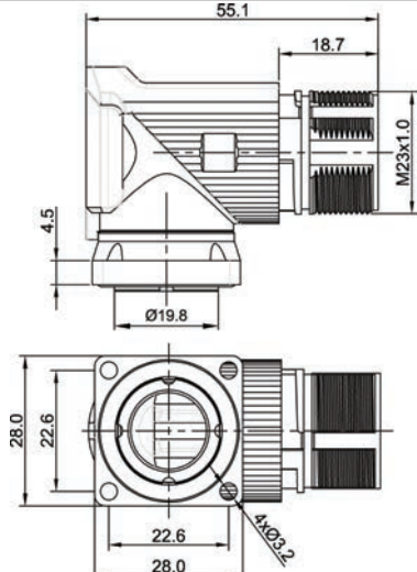
Receptacle, 90°, Checkmate™ Large Flange (28.0x28.0)
