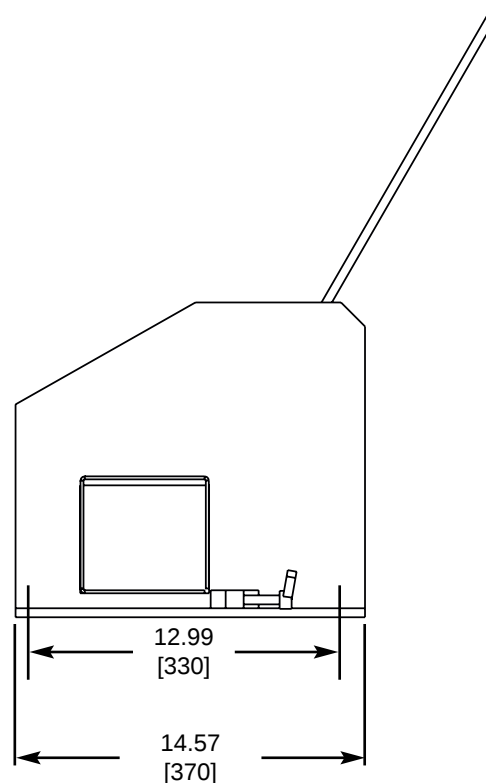
BDCT Side View with Mounting Dimensions
