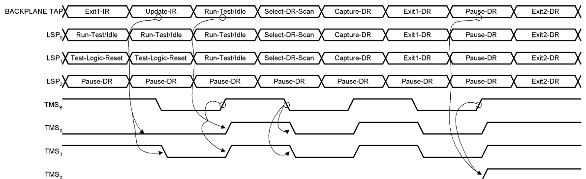
FIGURE 12. Synchronization of the Three Local Scan Ports
