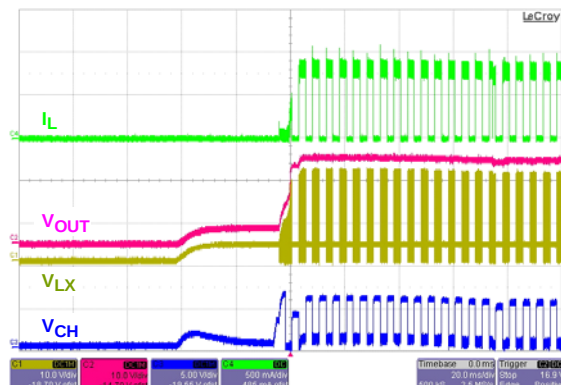
FIGURE 15. START-UP (50% DIRECT PWM DIMMING, V_{IN} : 3.7V, I_{CH} : 20mA, LEDs: 6P7S, f_{DIM} : 200Hz)
