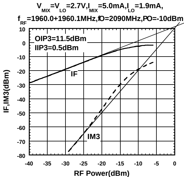
IF,IM3 vs. RF Power
