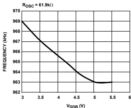
FIGURE 13. F_S vs V_{DD}
