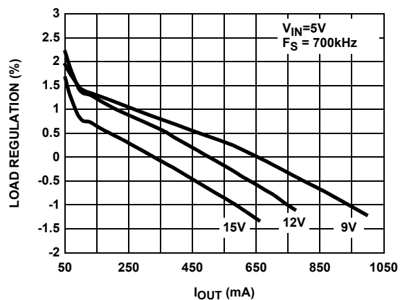
FIGURE 8. LOAD REGULATION
