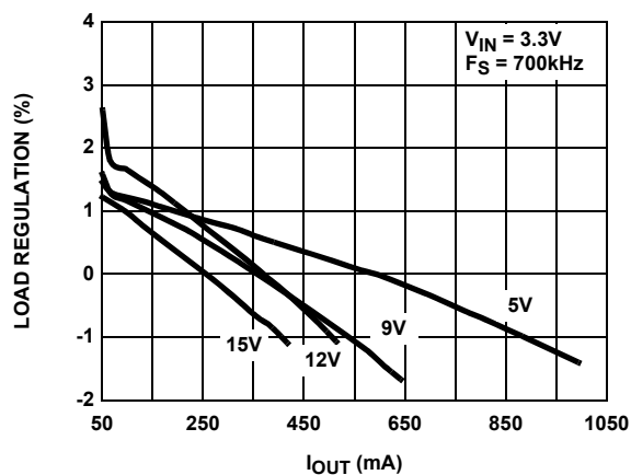
FIGURE 7. LOAD REGULATION
