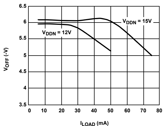
FIGURE 10. V_{OFF} vs I_{OFF}
