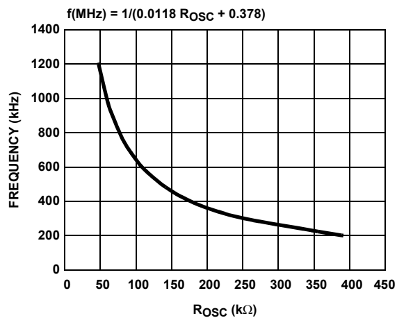
FIGURE 11. F_S vs R_{OSC}
