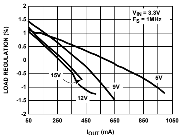
FIGURE 5. LOAD REGULATION
