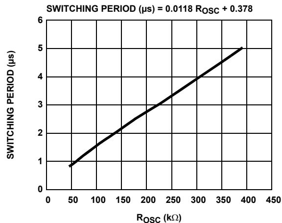
FIGURE 12. SWITCHING PERIOD vs R_{OSC}
