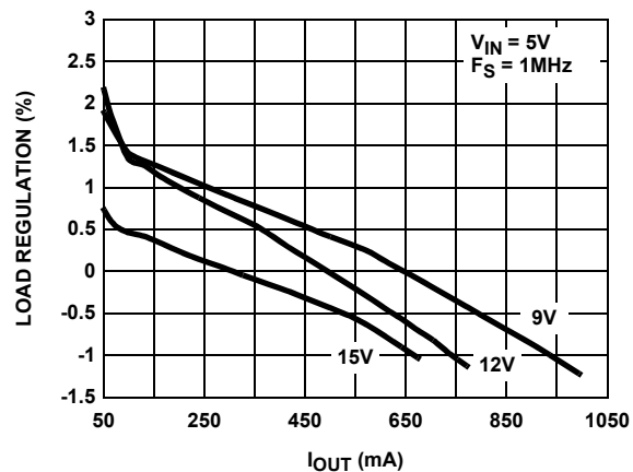
FIGURE 6. LOAD REGULATION
