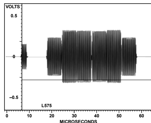
Figure 131. PAL Luma
