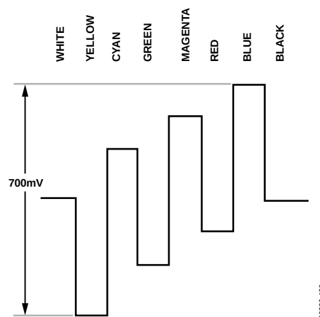
Figure 118. Pb Levels—PAL
