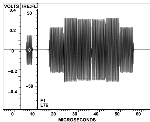
Figure 128. NTSC Luma
