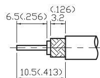
STRIPPING DIMENSION
