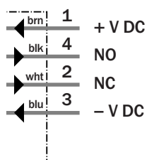
4 x 0.34 mm²
