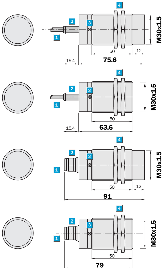
Dimensional drawing
