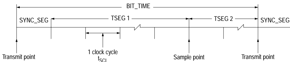
Figure 5-5 Segments within the bit time
