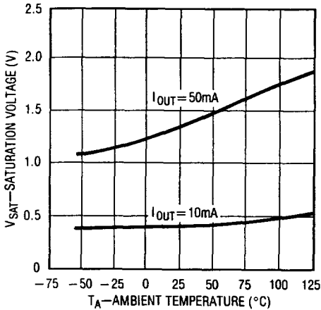
Output Transistor Saturation Voltage
