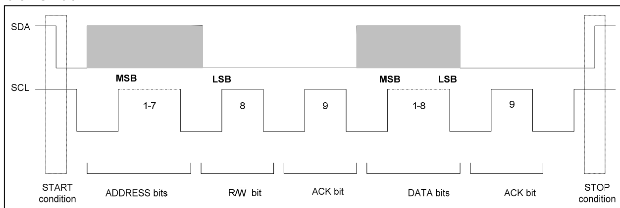
Figure 2: I²C Bus Write Protocol
