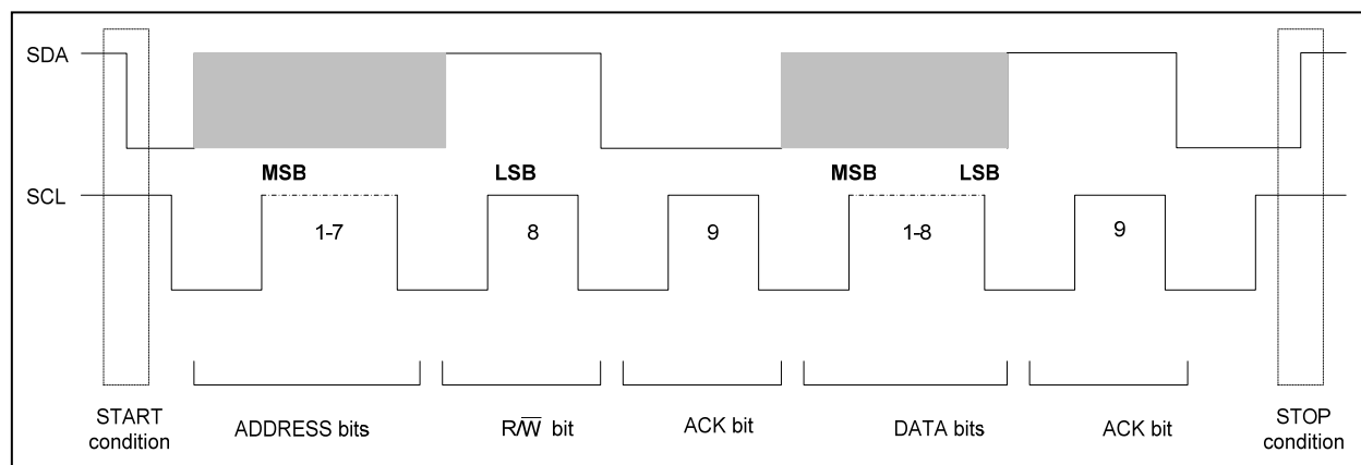
Figure 3: I²C Bus Read Protocol
