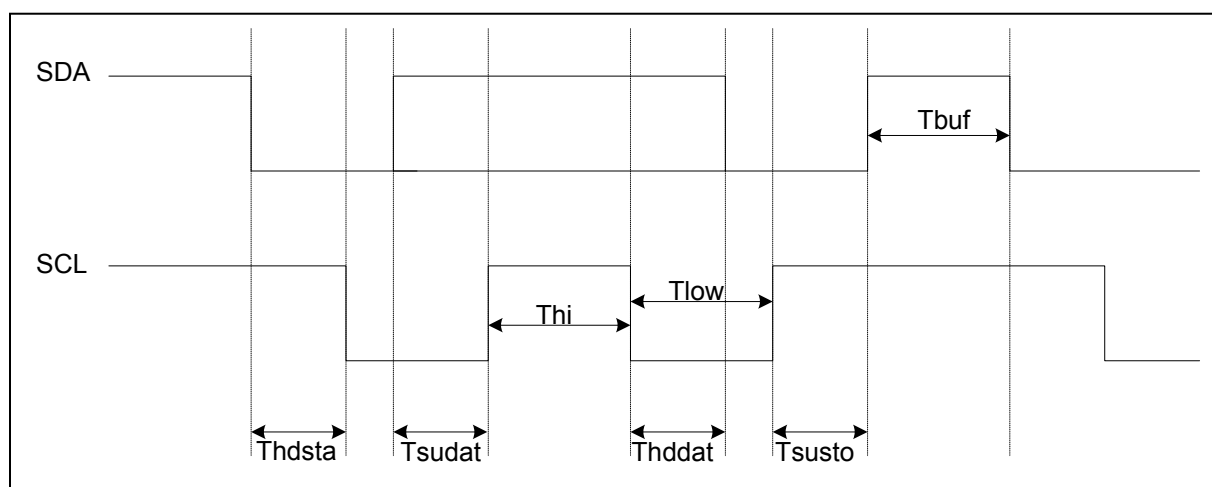
Figure 4: I²C Bus Timing Diagram
