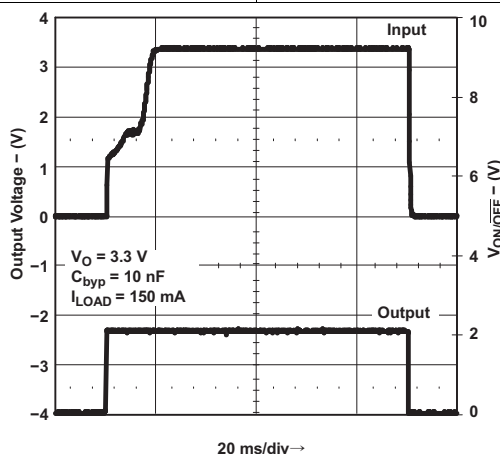
20 ms/div \rightarrow Figure 31. Turn-on Time
