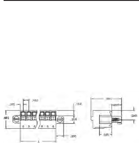
SCVF—.150" Pitch—Eared
