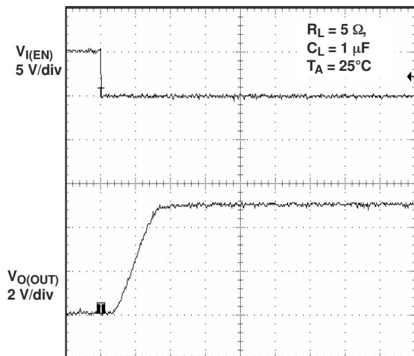
Figure 6-30. Turnon Delay and Rise Time With 1- \mu\text{F} Load
