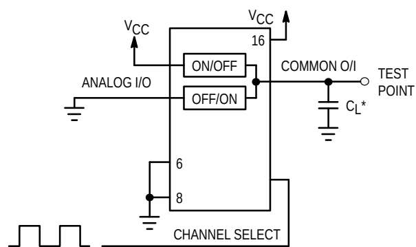
Figure 17. Propagation Delay, Test Set-Up Channel Select to Analog Out
