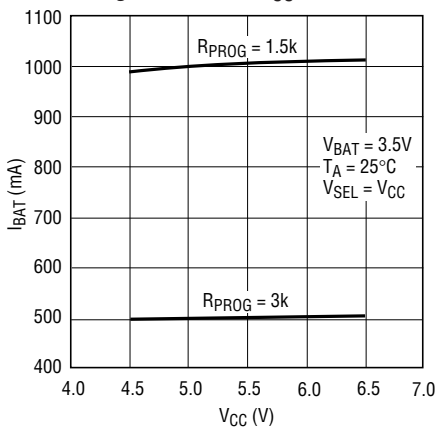
Charge Current vs V CC
