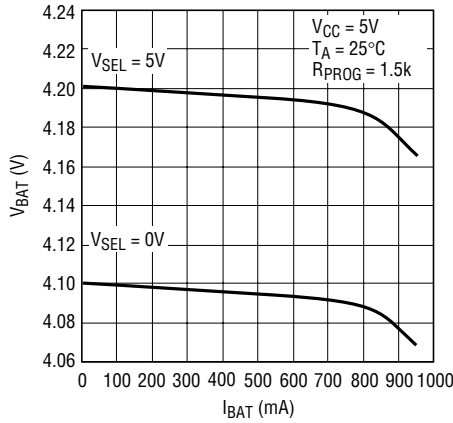
Battery Regulation Voltage vs Battery Charge Current
