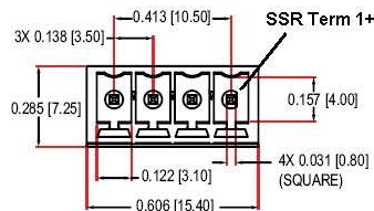
SUGGESTED MATING CONNECTORS/PLUGS
