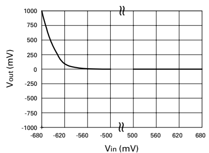
REC DC Transfer Characteristics
