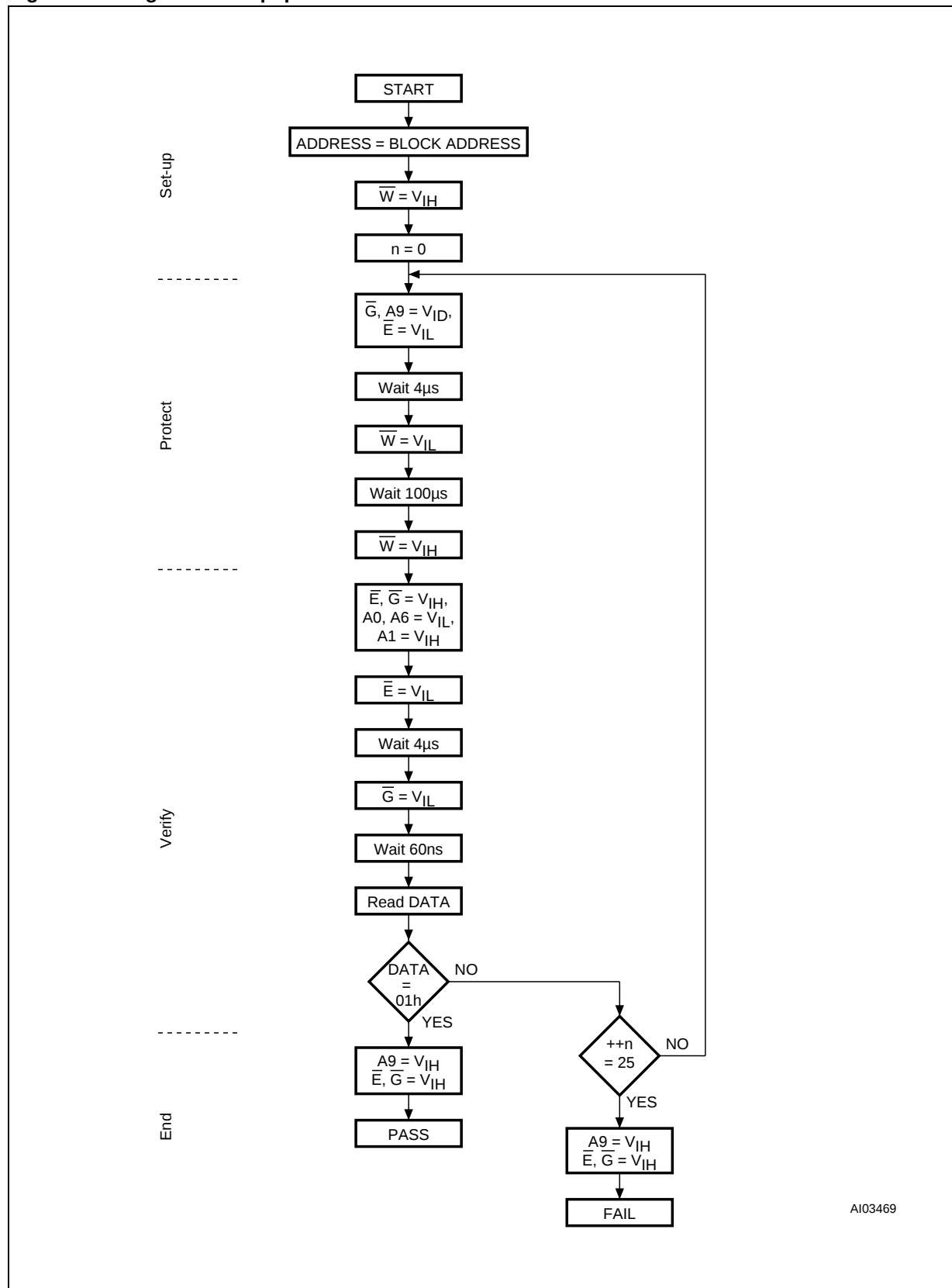
Figure 19. Programmer Equipment Block Protect Flowchart
