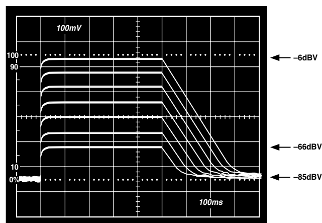
Figure 5a. RMS Level Detector Performance with C_{AVG} = 2.2 \mu F
