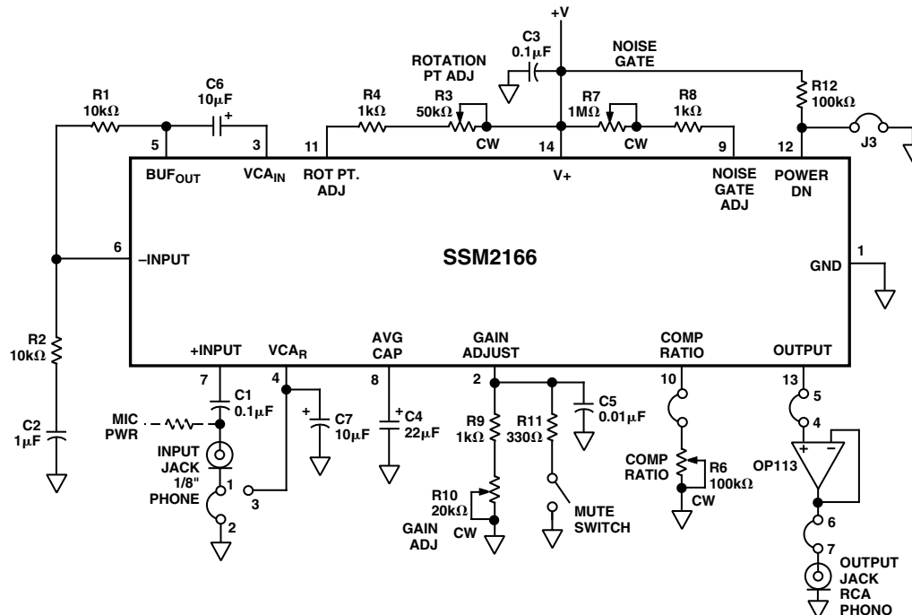
Figure 12. Evaluation Board
