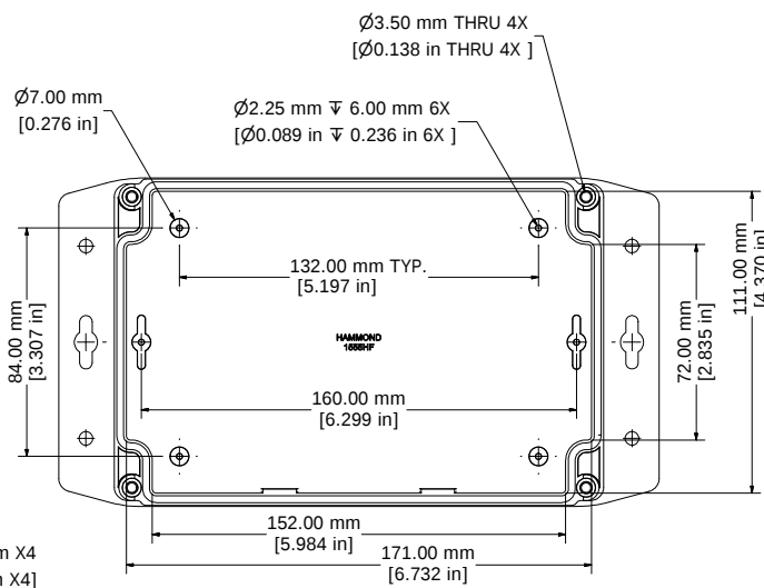
FLANGED LID INSIDE VIEW
