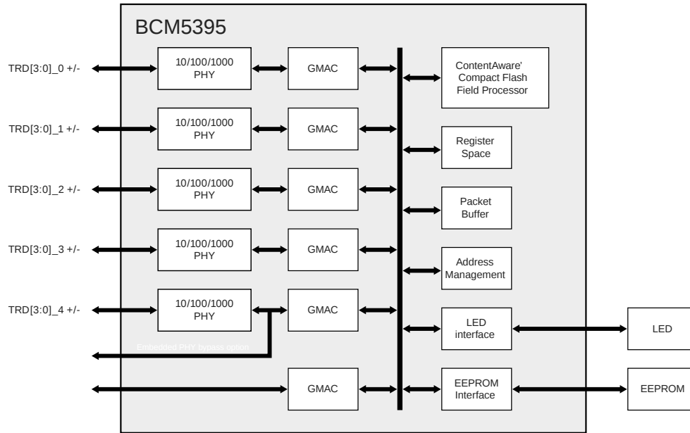
BCM5395 Block Diagram
