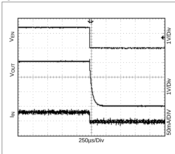
Figure 45. Shutdown
