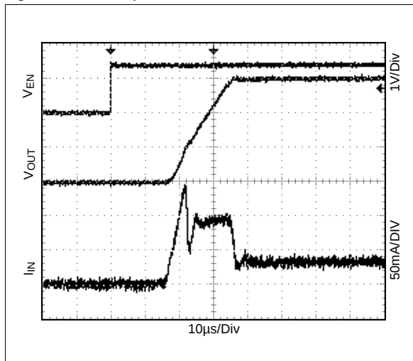
Figure 44. Startup
