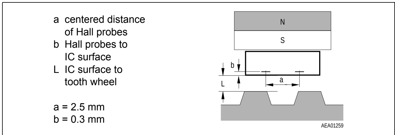
Figure 5 Sensor Spacing
