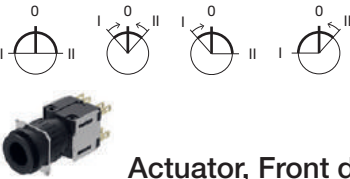
Actuator, Front dimension Ø 18 mm
