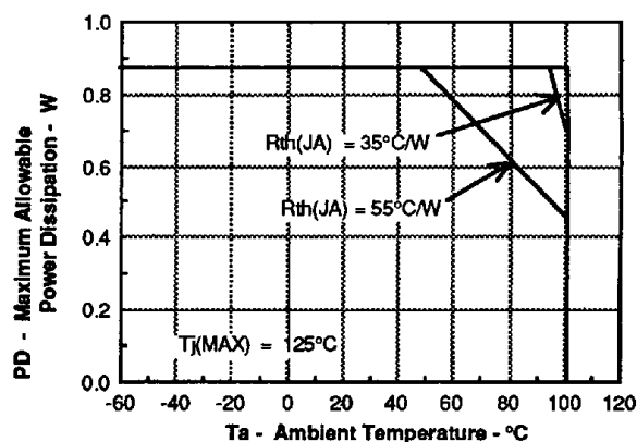
FIGURE 2. MAX. ALLOWABLE POWER DISSIPATION VS. TEMPERATURE
