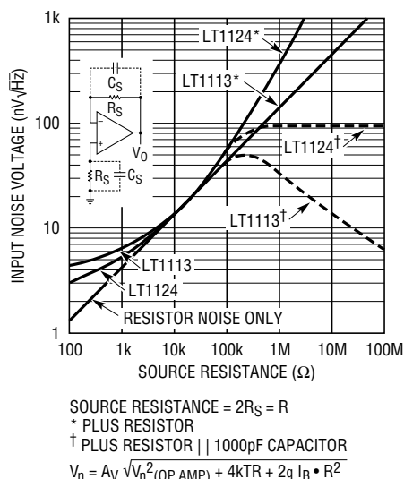
Figure 1. Comparison of LT1113 and LT1124 Total Output 1kHz Voltage Noise Versus Source Resistance
