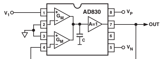
V_{OUT} = V_I GAIN OF 1 (c)
