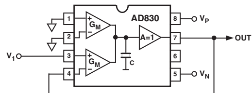
V_{OUT} = V_I OP AMP CONNECTION (b)
