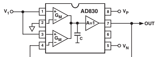
V_{OUT} = 2V_I RESISTORLESS GAIN OF 2 (a)
