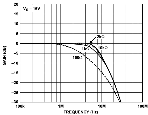
Figure 28. Gain vs. Resistive Load
