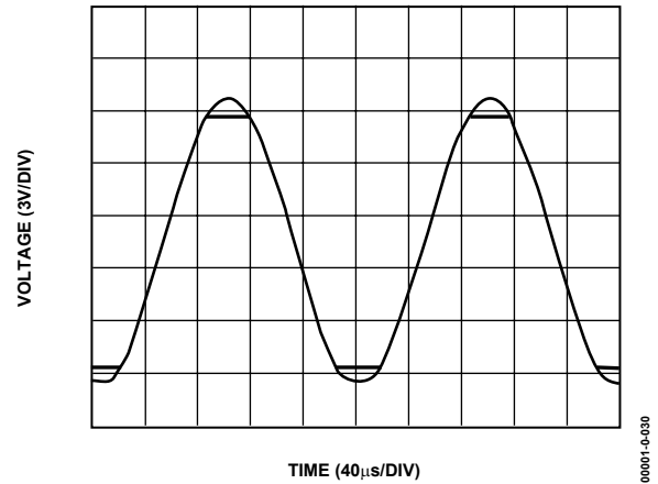
Figure 30. No Phase Reversal
