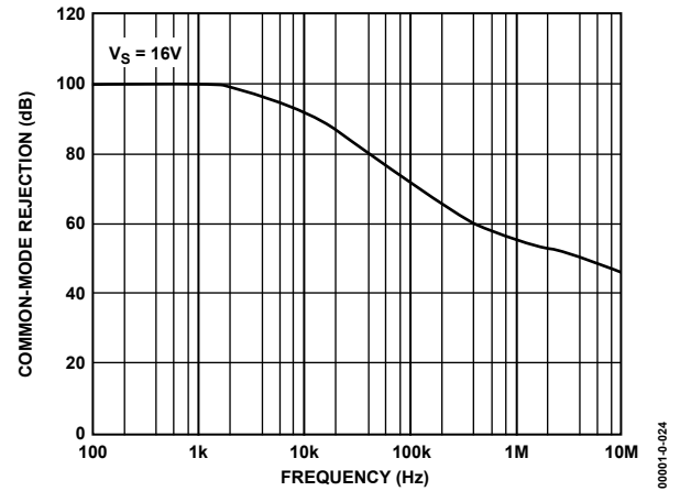
Figure 24. Common-Mode Rejection vs. Frequency
