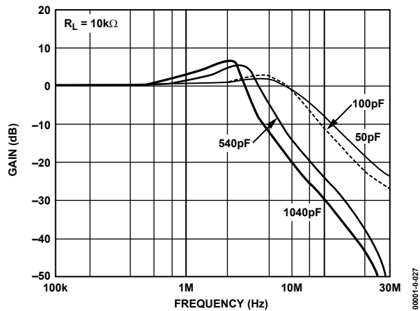
Figure 27. Gain vs. Capacitive Load
