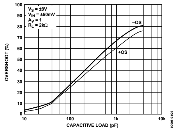
Figure 26. Overshoot vs. Capacitive Load
