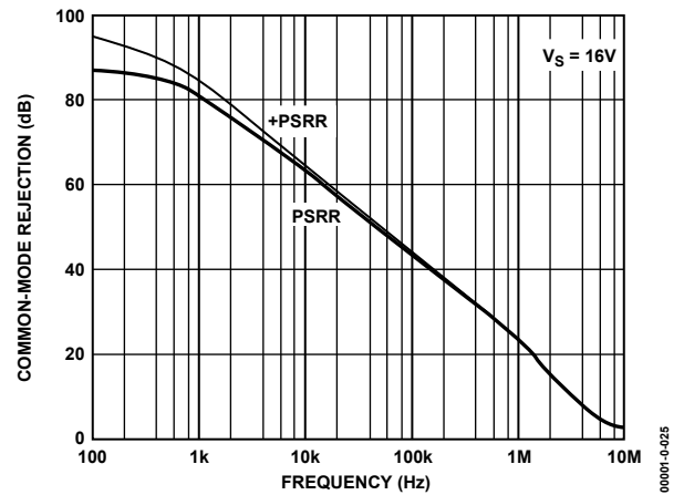
Figure 25. Common-Mode Rejection vs. Frequency
