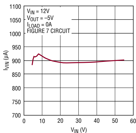
Pulse-Skipping Mode Input Current Over Input Voltage (No Load)
