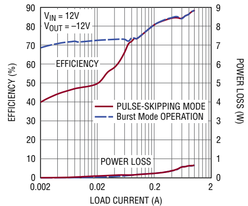
-12V Efficiency
