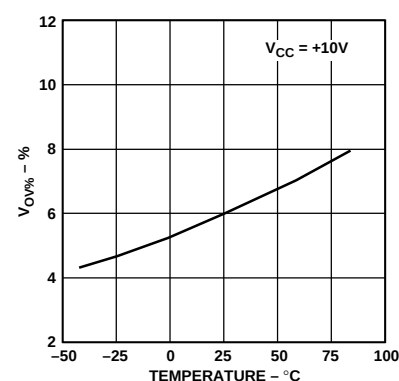
Figure 19. Overvoltage Comparator Threshold ( V_{OV\%} ) vs. Temperature
