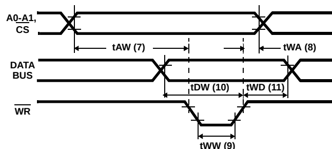
FIGURE 30. WRITE TIMING
