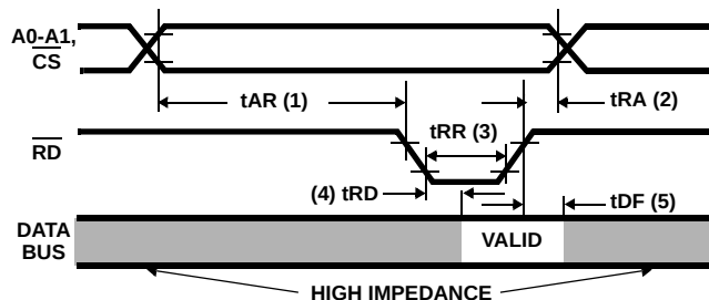
FIGURE 31. READ TIMING
