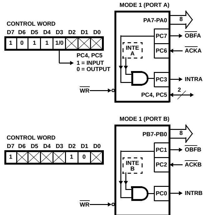
FIGURE 8. MODE 1 OUTPUT
