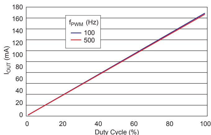
Figure 8. PWM pin dimming linearity.
