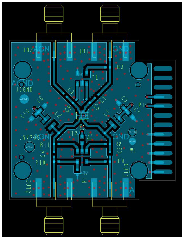
Figure 26. Evaluation Board Layout, Top Layer
