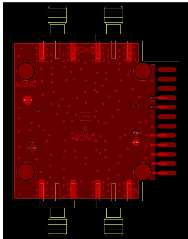
Figure 27. Evaluation Board Layout, Bottom Layer
