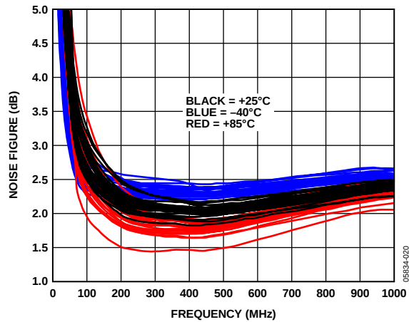
Figure 21. Noise Figure Temperature Distribution, V_{POS} = 3\text{ V}
