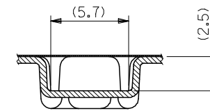
SECT:X-X (SCALE 4:1)
