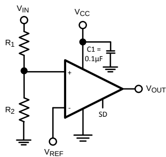
Figure 1. Threshold Detector
