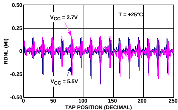
FIGURE 5. RDNL vs TAP POSITION IN RHEOSTAT MODE FOR 10k\Omega (W)
