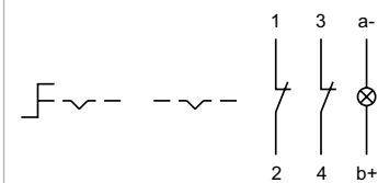
Wiring diagram 18
