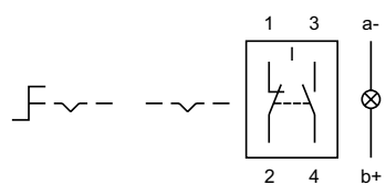
Wiring diagram 23
