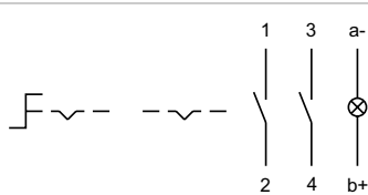
Wiring diagram 19
