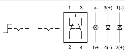
Wiring diagram 21
