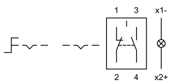
Wiring diagram 22
