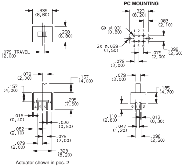
OS202011MS2QS1 DPDT
