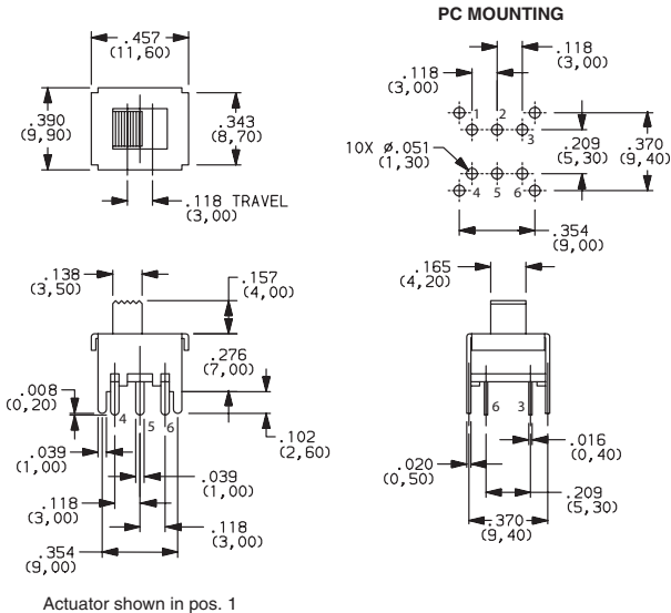
OS202013MT5QN1 DPDT
