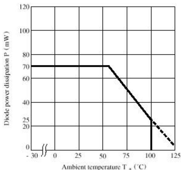
Diode Power Dissipation vs. Ambient Temperature
