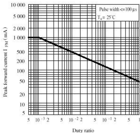
Peak Forward Current vs Duty Ratio
