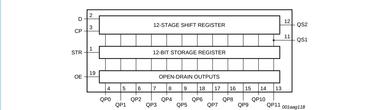
Fig 2. Functional diagram
