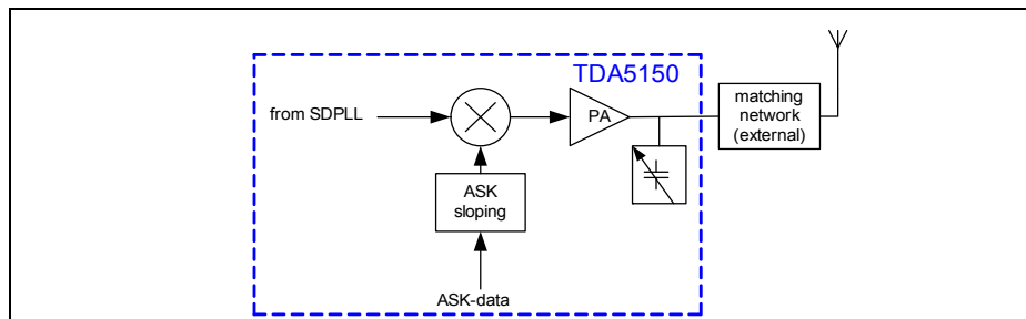
Figure 16 Transmitter Blocks
