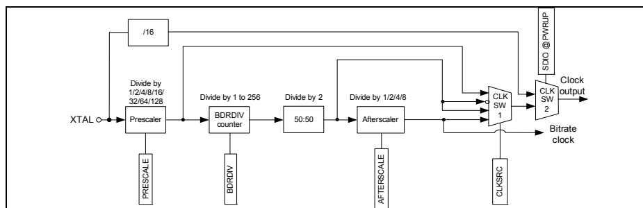
Figure 13 Bit-Rate Divider
