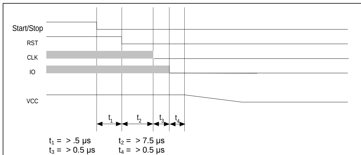
Figure 9: Deactivation Sequence
