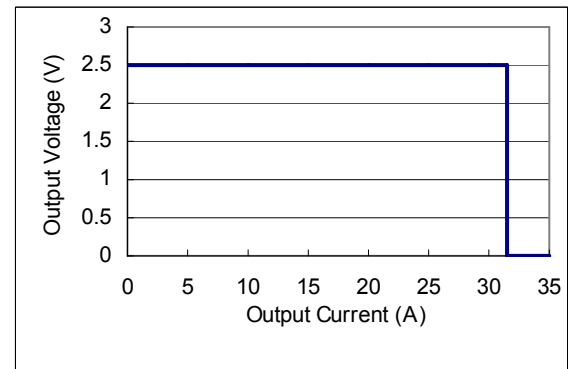
Fig. 11 Typical output over-current of AVO75-48S2V5
