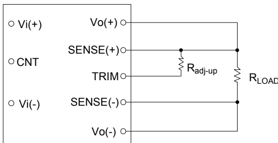
Fig. 73 Trim up circuit
