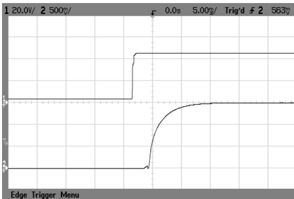
Fig. 59 AVO75-48S1V5 typical start-up from power on
