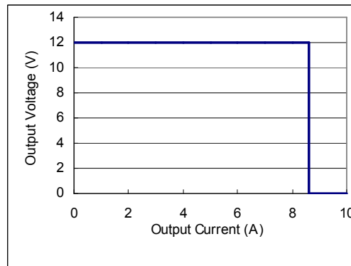
Fig. 14 Typical output over-current of AVO75-48S12
