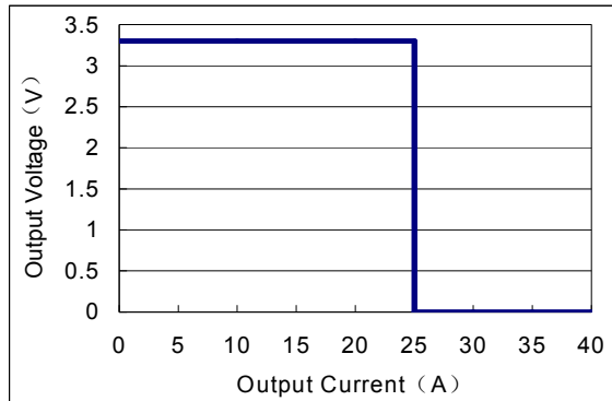
Fig. 12 Typical output over-current of AVO75-48S3V3
