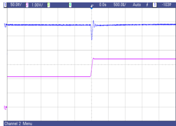
Fig. 23 AVO75-48S1V2 typical transient response to step increase in load from 50% to 75% of full load, room temperature, 48Vdc input
