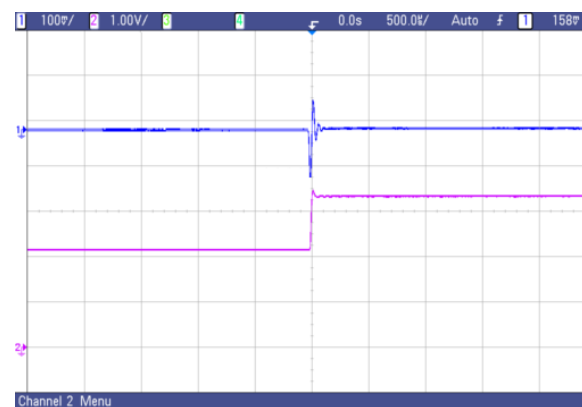
Fig. 33 AVO75-48S1V8 typical transient response to step increase in load from 50% to 75% of full load, room temperature, 48Vdc input ( \Delta I_o/\Delta t=1A/1\mu s )
