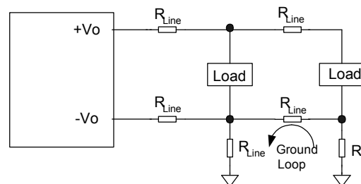
Fig. 77 Ground loops
