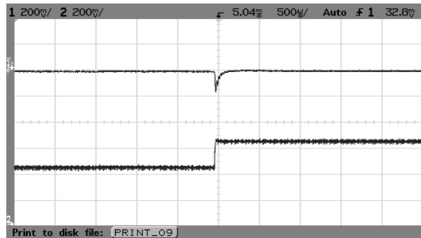
Fig. 49 AVO75-48S12 typical transient response to step increase in load from 50% to 75% of full load, room temperature, 48Vdc input ( \Delta I_o/\Delta t=1A/1\mu s )
