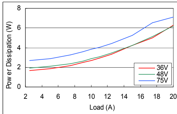
Fig. 19 Typical power dissipation of AVO75-48S3V3
