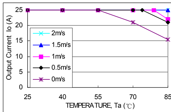
Fig. 84 AVO75-48S1V5 output power derating Airflow direction from -Vin to +Vin; V_{in} = 48V
