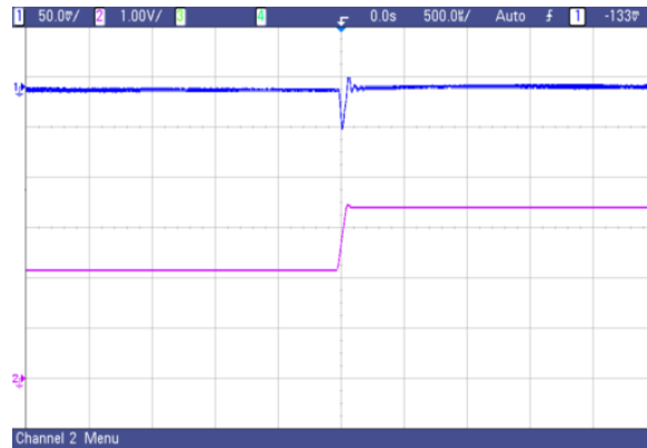
Fig. 31 AVO75-48S1V8 typical transient response to step increase in load from 50% to 75% of full load, room temperature, 48Vdc input ( \Delta I_o/\Delta t=0.1A/1\mu s )
