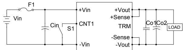
Fig. 79 Typical application
