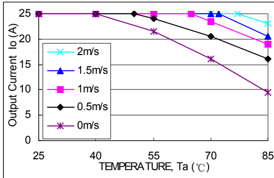
Fig. 86 AVO75-48S2V5 output power derating Airflow direction from -Vin to +Vin; Vin=48V
