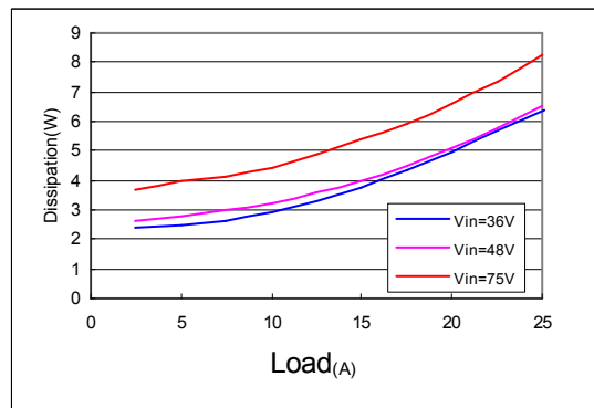
Fig. 18 Typical power dissipation of AVO75-48S2V5
