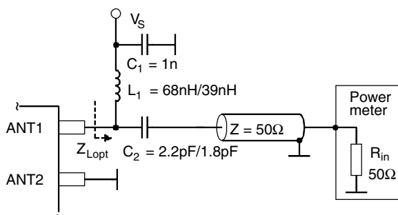
Figure 4-6. Output Power Measurement Atmel ATA8404/ATA8405
