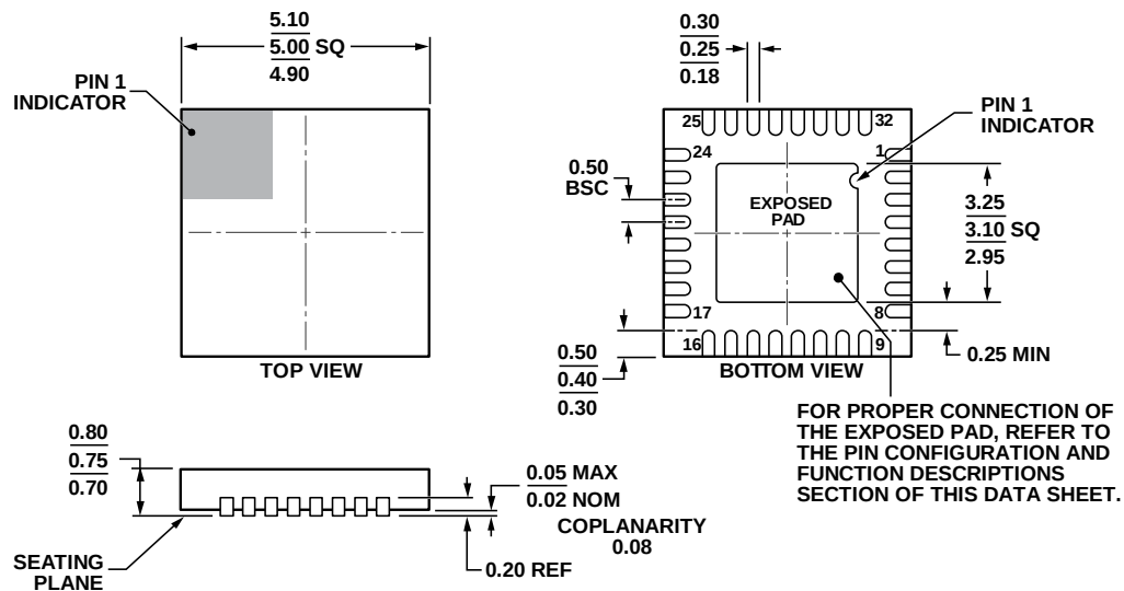
Figure 60. 32-Lead Lead Frame Chip Scale Package [LFCSF_WQ] 5 mm × 5 mm Body, Very Very Thin Quad (CP-32-7)
